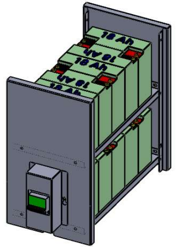
NC00 - 18Ah x 10
