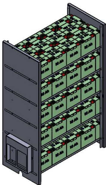
NC51 - 18Ah x 110
