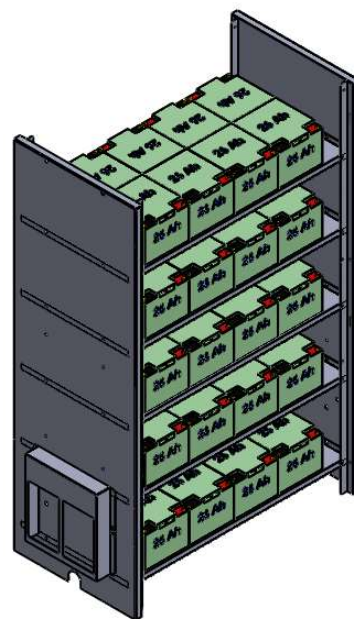
NC51 - 26Ah x 40
