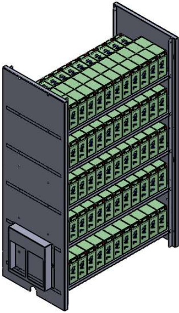
NC51 - 7Ah x 180
