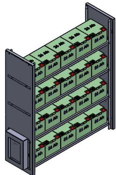
NC30 - 26Ah x 20
