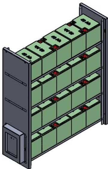
NC30 - 40Ah x 20
